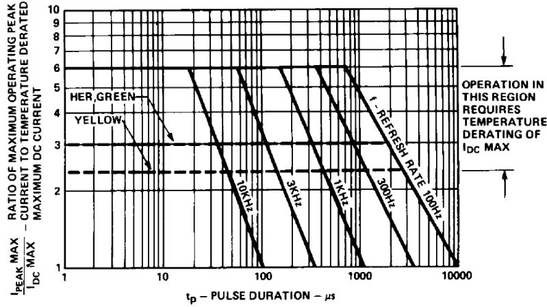
Figure 6. Maximum Allowed Peak Current vs. Pulse Duration.
